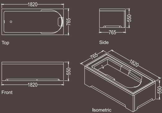
DRAWING & PRE-INSTALLATION
