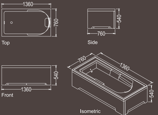
DRAWING & PRE-INSTALLATION
